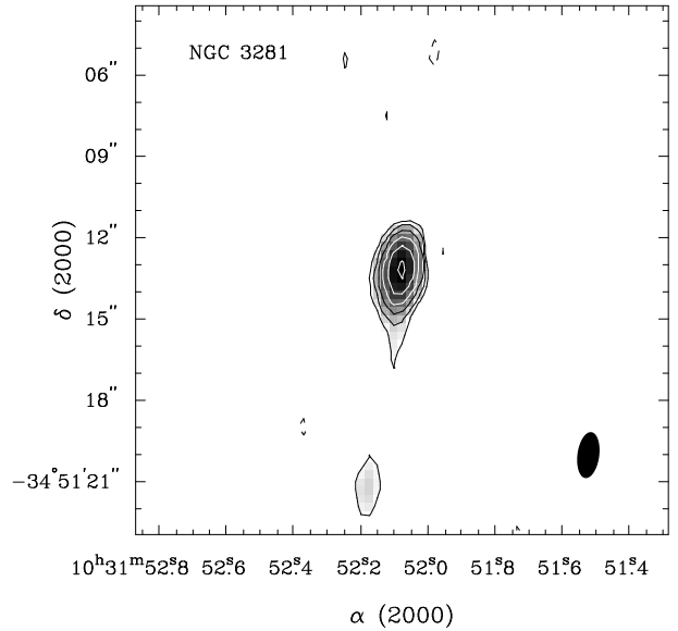
Fig. 8. NGC 3281. Contours: -0.9, -0.5, 0.5, 0.9, 1.9, 3.7, 7.2, 14.2 mJy beam -1
